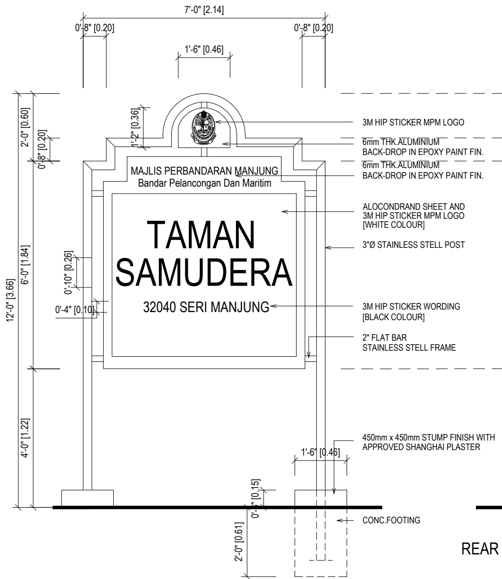
FRONT ELEVATION OF SIGNBOARD [TYPE A] SCALE : 1/2" TO 1'-0"
