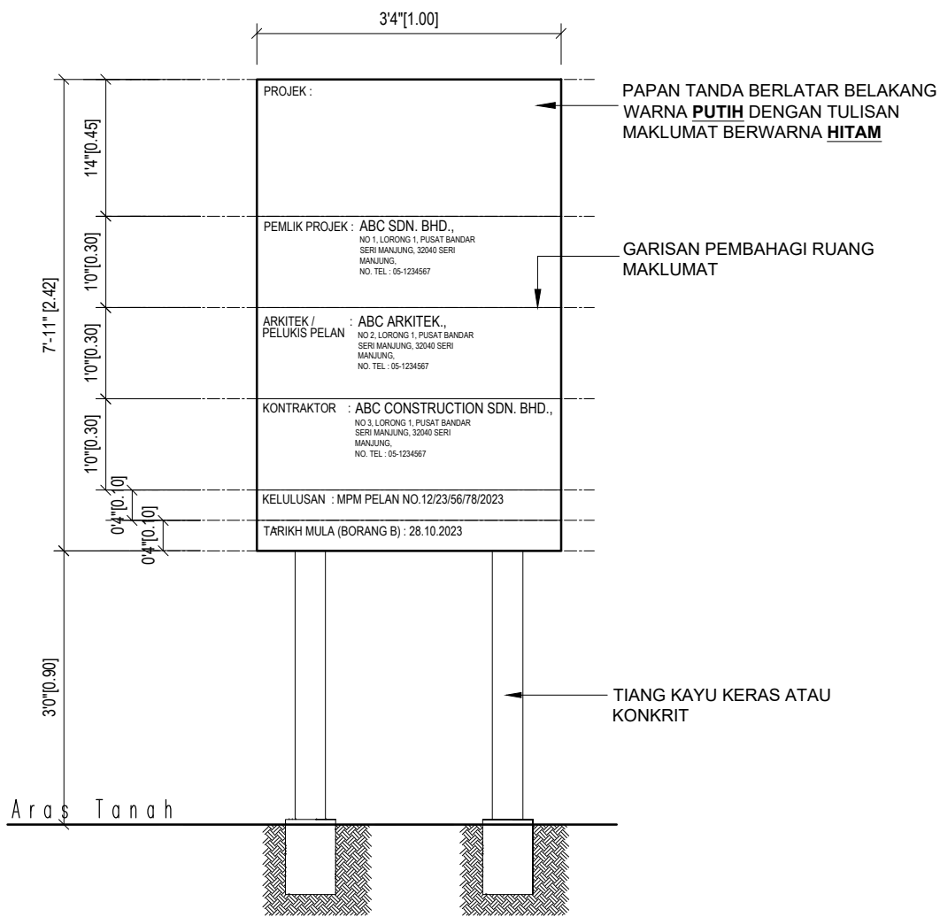
FRONT ELEVATION SCALE : 1/2" TO 1'-0"
